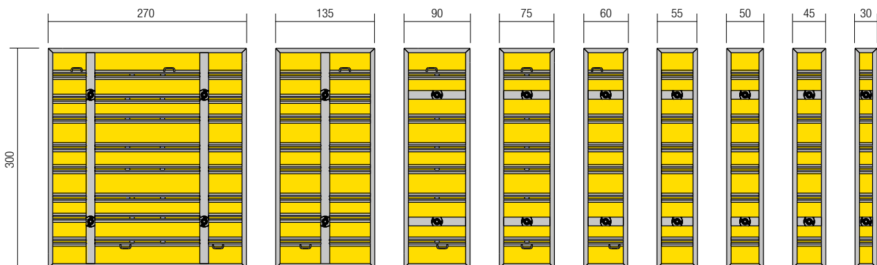
Panel size-grid of Framax Xlife plus 3.00 m / sizes in cm
