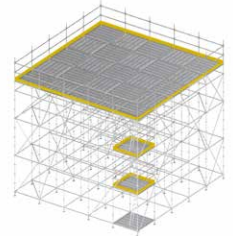
Birdcage scaffold
