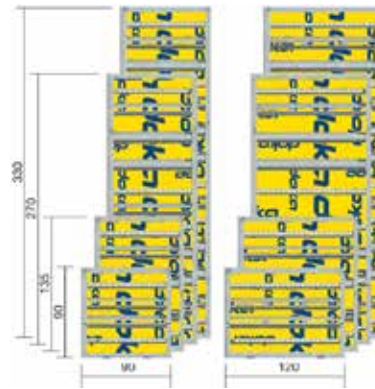
Framax Xlife universal panels are available in widths of 90 cm and 120 cm and in panel heights of 90 cm, 135 cm, 270 cm and 330 cm.
