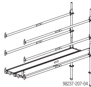
Base, right buttress bay
