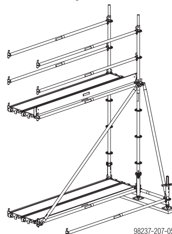
Base, right buttress bay
