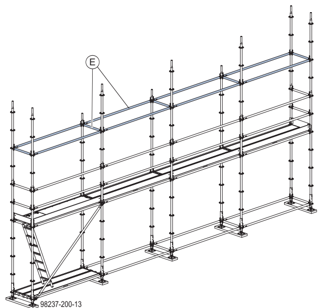
E Transverse ledger and longitudinal ledger
