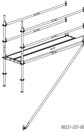
Lift, left buttress bay
