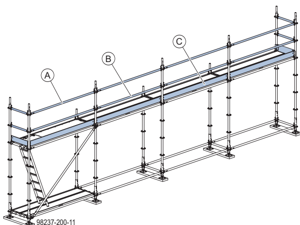
A Ledge as top guardrail
