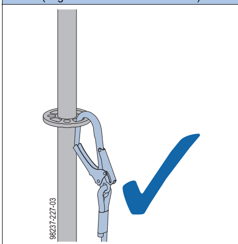
Attachment to Ringlock rosette permitted (large and small holes in rosette)
