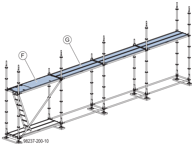
F Alum. hatch deck
