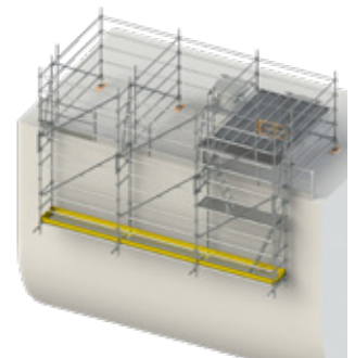
Hanging Scaffolding
