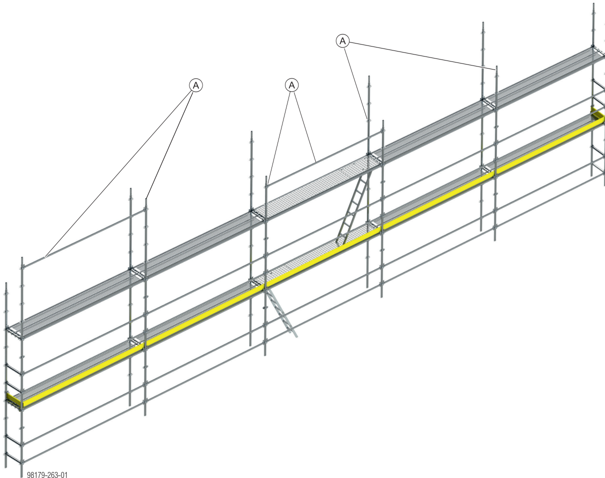
A Anchor points for PPE
