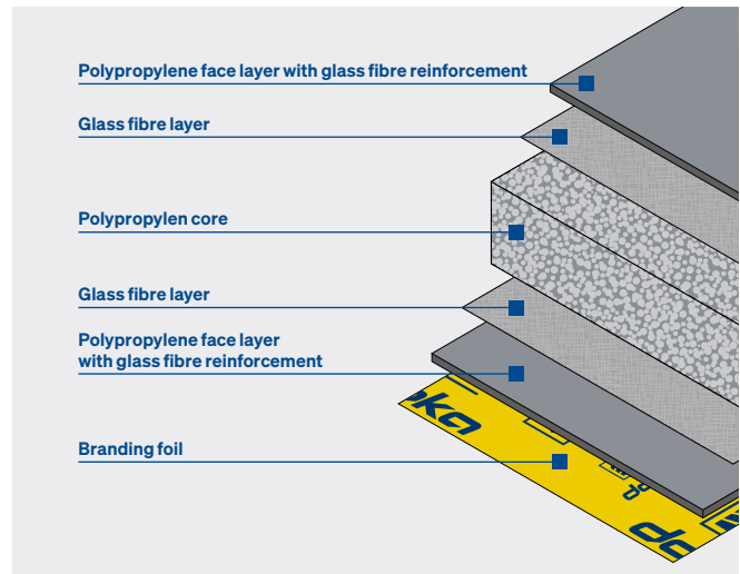
Structure of Xlife top sheet
