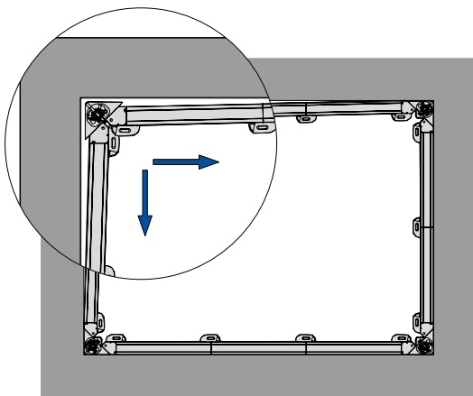
The formwork is detached very quickly, with a stripping play of 6 cm
