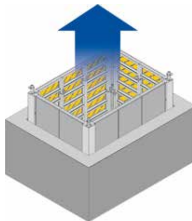
The shaft formwork is lifted in one piece
