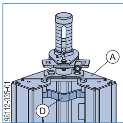
A Framax stripping corner I
