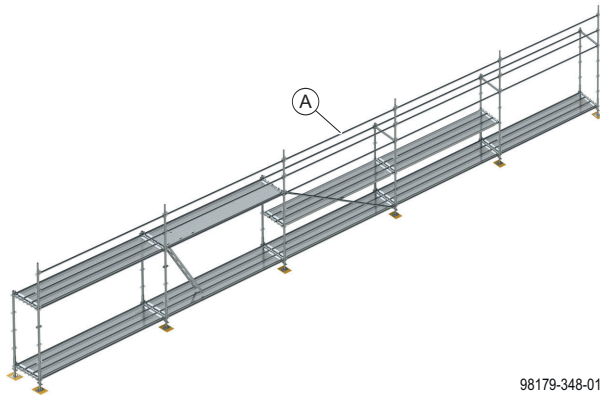
A Advanced guardrail assembled with Ringlock Ledgers
