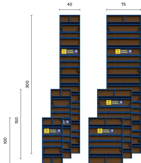
Universal panels for columns and corners with panel connections every 5cm.
