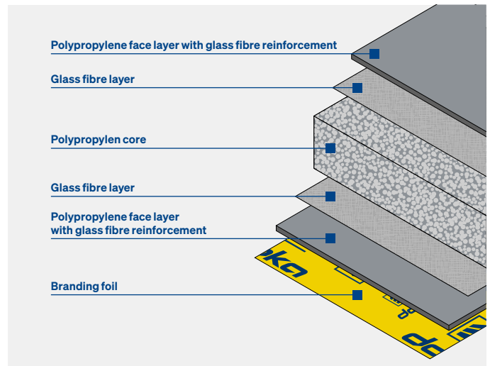
Structure of Xlife top sheet
