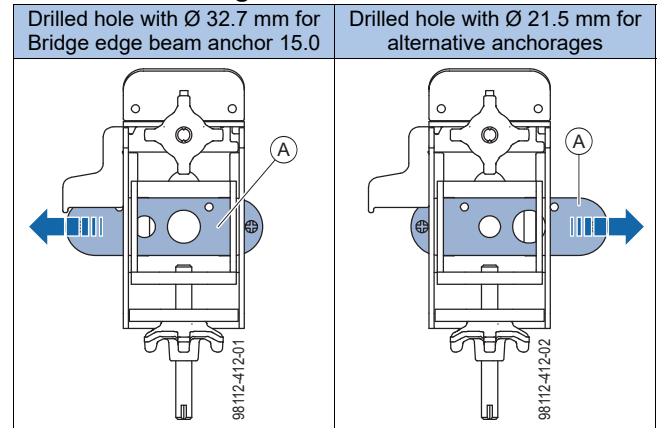
A Plate for pushing to the respective drilled hole
