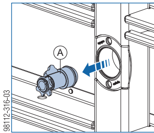
A Framax Xlife plus form-tie nut I 20.0
