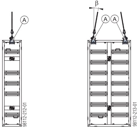
A Welded-on metal plate
