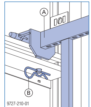
Anti-liftout guard
