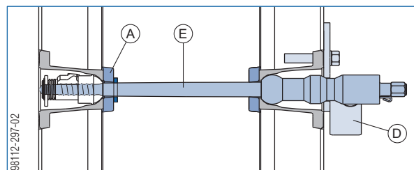
A Framax Xlife plus fair-faced concr. cone 87mm
