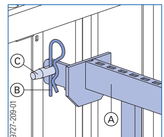
Anti-liftout guard
