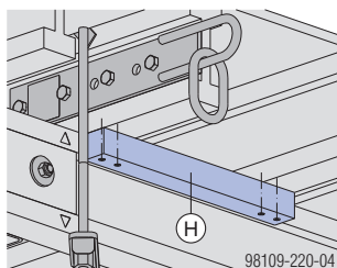
H Kantholz ca. 2x2 (5 x 5 cm) (B x H)
