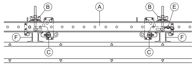
A Multi-purpose waling (WS10, WU12, WU14 or WU16)
