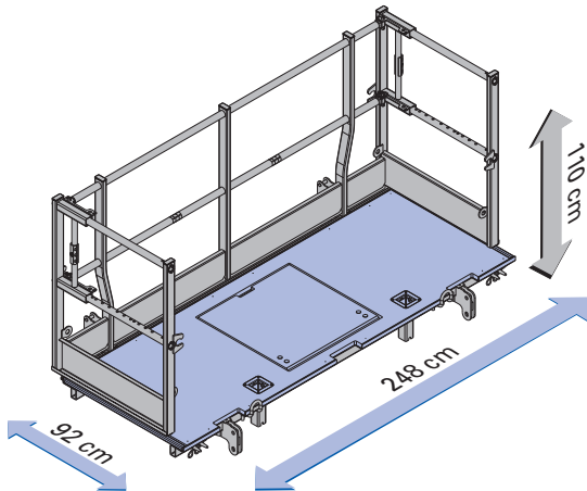
Xsafe plus platform 2.50m with side railings (or without side railings)
