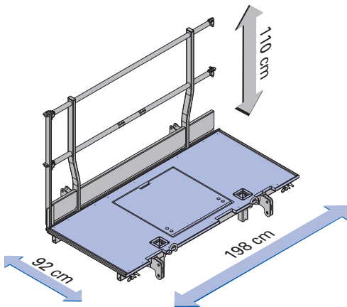
Xsafe plus platform 2.00m (Xsafe plus side railings can be added)
