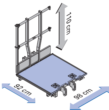
Xsafe plus platform 1.00m (Xsafe plus side railings can be added)
