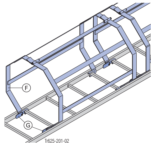
F Rückenschutz XS 1,00m
