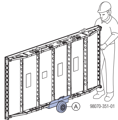
A M-Timber trolley 170 mm-CT
