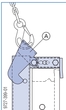
A Safety hook
