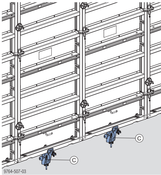
C Wall-formwork support angle 2G or Wall-formwork support angle
