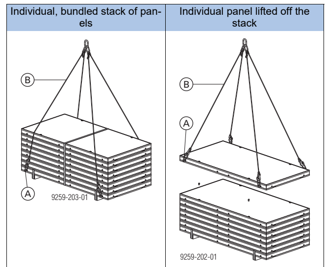
A Framax transport bolt B Doka 4-part chain 3.20m
