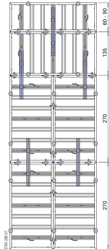
Formwork height: 735 and 765 cm
