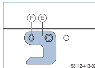
Parking position for wooden planks
