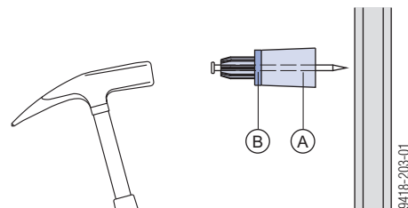
A Nagelkonus 15,0
